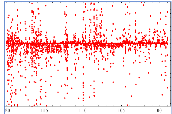
Figure 4. Bifurcation diagram.
